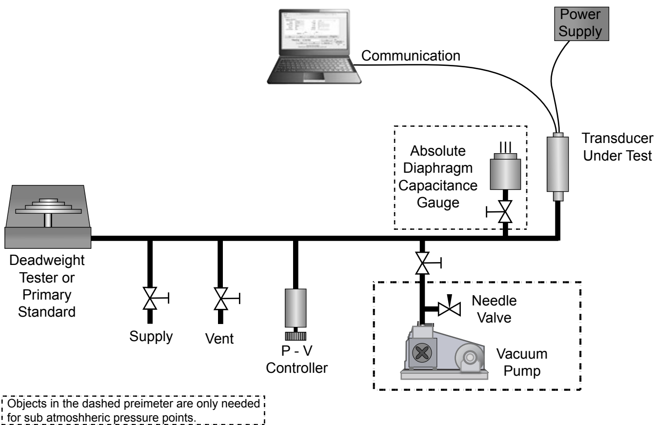
Figure 7.2.5 - Calibration Setup
